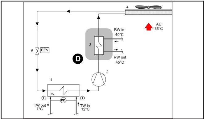
D - Partial recovery device
