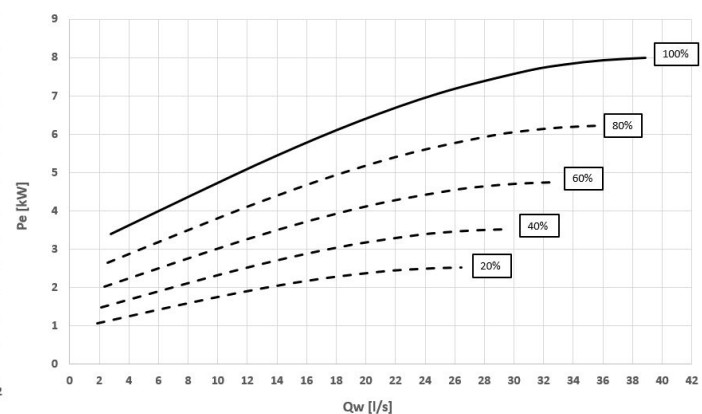
Power input - Size 280.2 ÷ 320.2
