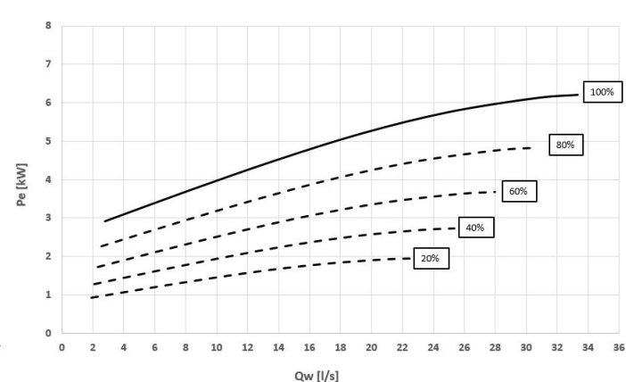
Power input - Size 220.2 ÷ 260.2
