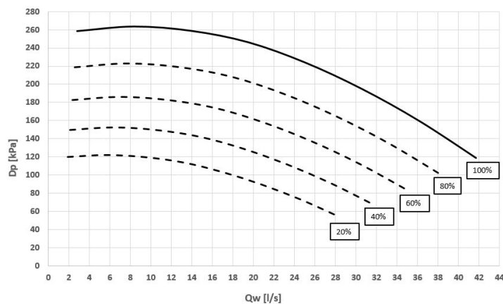
Head - Size 340.2
