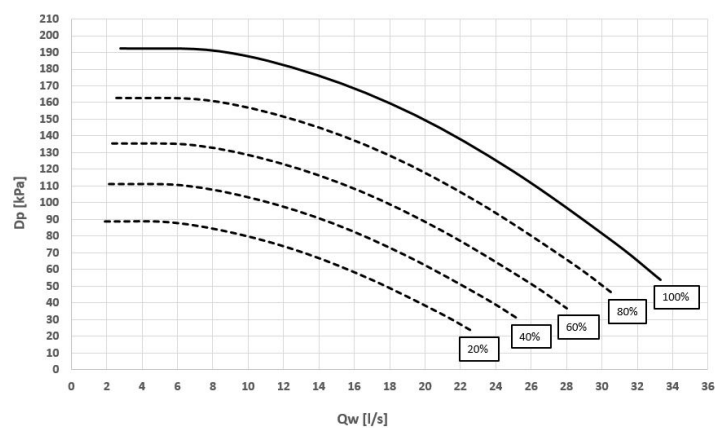
Head - Size 220.2 ÷ 260.2
