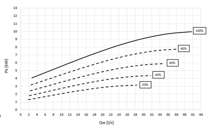
Power input - Size 340.2
