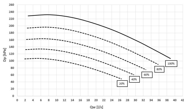
Head - Size 280.2 ÷ 320.2
